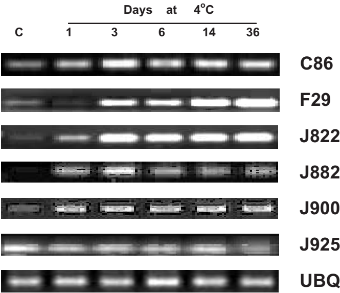
Fig. 3. Gene expression profile for selected genes. Transcript levels of cold-regulated genes C86, a glycine-rich protein; F29, a receptor-like kinase; J822, guanine nucleotide regulatory protein; J882, an inorganic pyrophosphatase; J900, a calcium-binding EF-hand protein; J925, a GTP-binding protein measured by RT-PCR. Seedlings of freezing-tolerant winter cultivar ‘Clair’ were either kept at 22 °C (C) or grown at 4 °C for the periods indicated. Their total RNAs were extracted and used for RT-PCR with gene-specific primers as described in Materials and methods.
