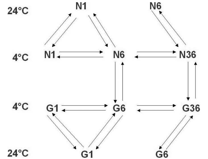
Fig. 1. The experimental design is based on the series of pairwise comparisons. Numbers indicate the number of days plants were grown at the indicated experimental temperatures. Before day 1 of the experiment, all plants had been germinated and grown for 7 days at 24 °C. N, winter wheat ‘Norstar’; G, spring wheat ‘Glenlea’.
